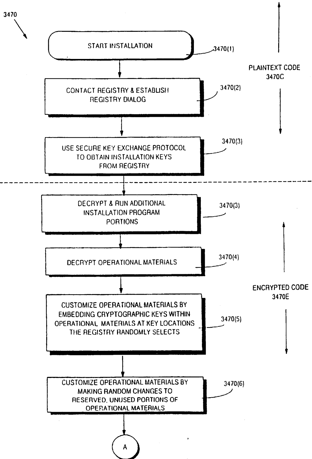
Fig. 69B Example Installation Routine
